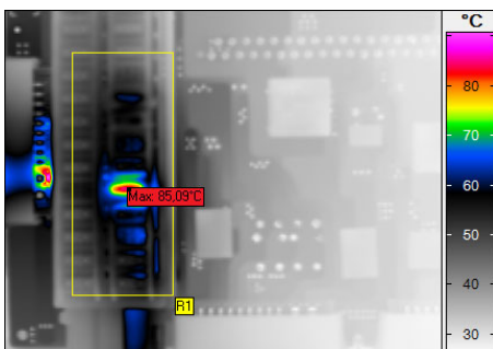
Abb. 2: 5x digital zoom of thermal image of fuse block
