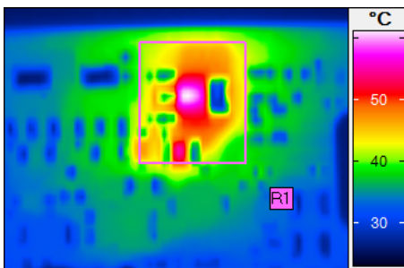
Abb. 1: 5x digital zoom of thermal image with hotspot - PCB
